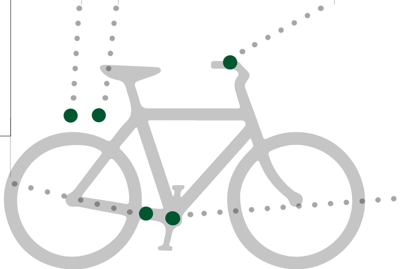
Center motor, torque sensor and f/coaster brake. 50378-38. Standard chainwheel for internal hub.
